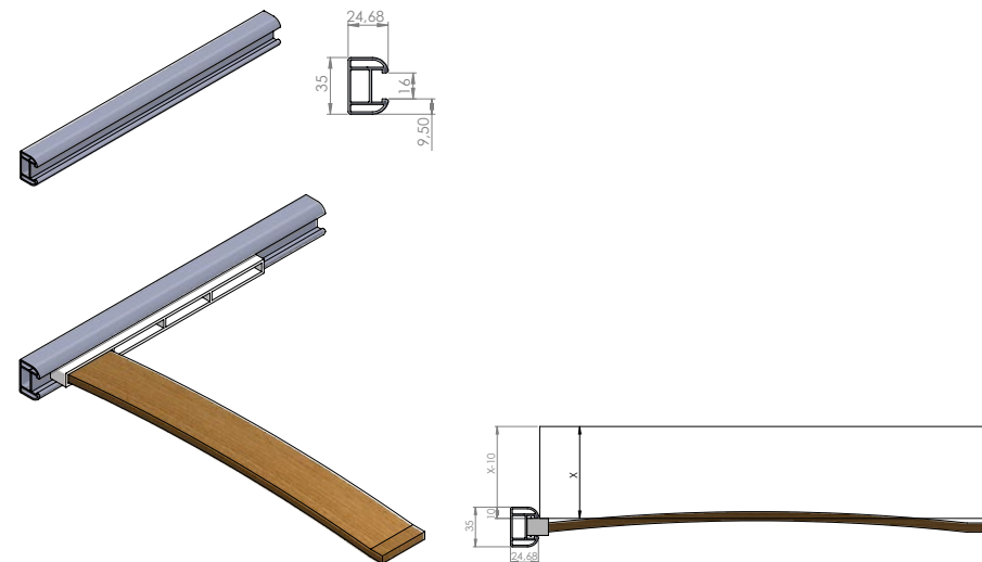
Detail H - Standard Slat Holder
