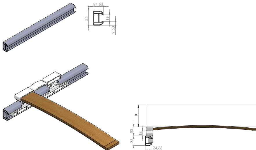
Detail G - Comfort Slat Holder
