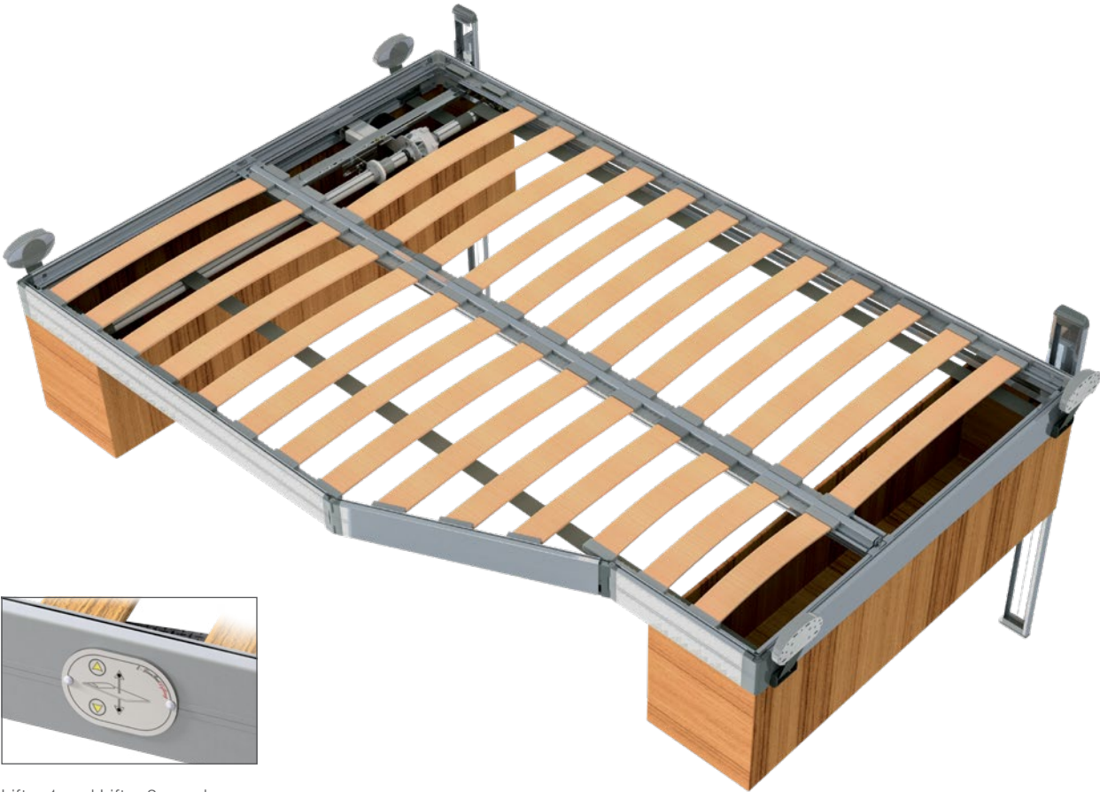
Lifter 1 and Lifter 2 panels can be embedded into the bed frame
