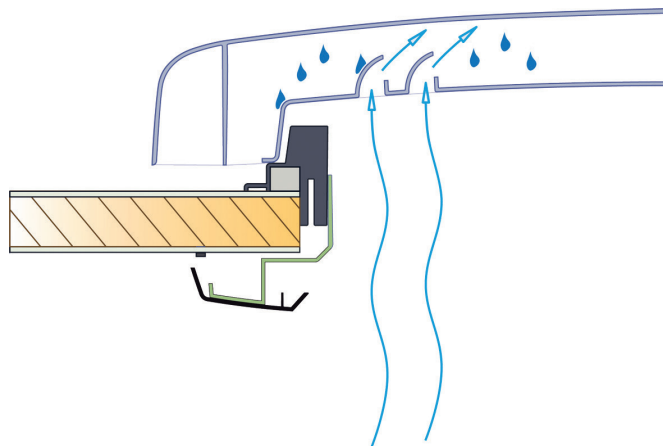
Aerodynamic dome with a permanent airflow
