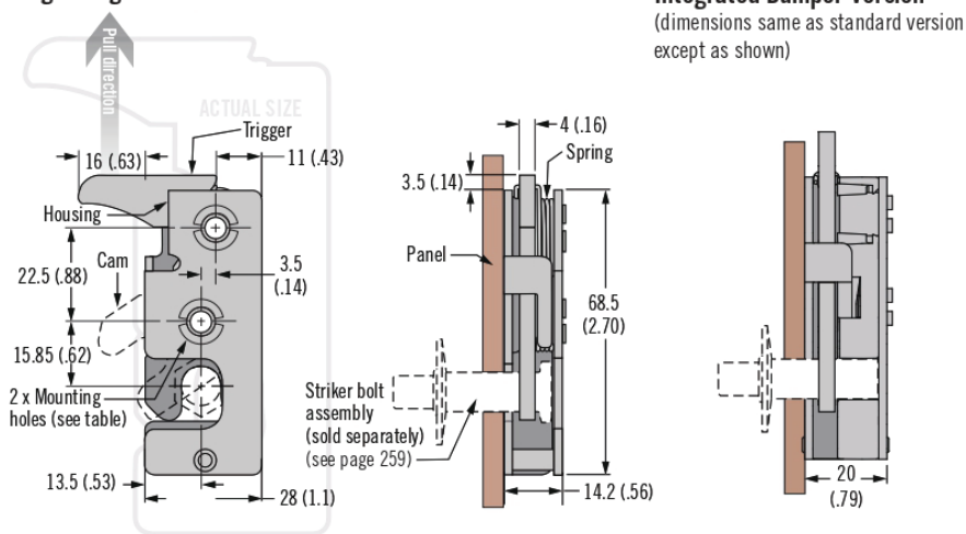
Single Stage - Hand Actuation
