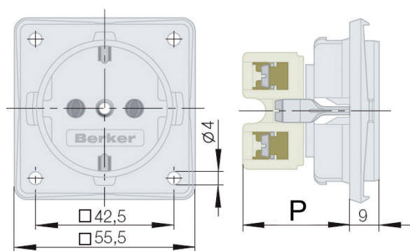
Standard dimensions for socket range
