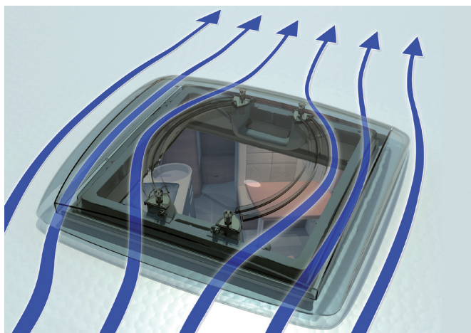
Aerodynamic dome with a permanent airflow
