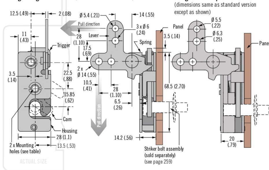
Single Stage - Hand Actuation
